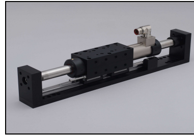
AD09 mechanical stops with PA01 wipers on HA01
