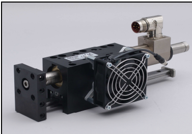
AD02 cooling fan adaptor for HM01 & HA01
