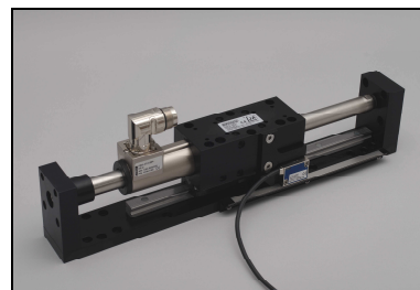
AD06 mounting set & magnetic scale with external incremental positioning sensor for HM01
