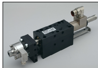
AD01 adaptor for force transducer HBM U2B with HM01-37 & HM01-48
