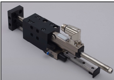
AD05 pneumatic brake for HM01
