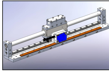
AD56 mounting set & magnetic scale with external inkremental positioning sensor for QM02
