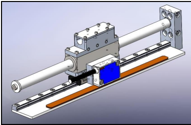
AD56 mounting set & magnetic scale with external inkremental positioning sensor for QM02
