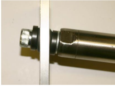
Function: Ball and socket washers adjust for angular offset between linear motor slider and Payload. (A spring washer should be used as well.)
